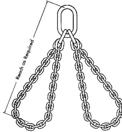
DOUBLE BASKET
