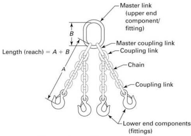
(a) Quadruple-Leg Bridle Sling Components
