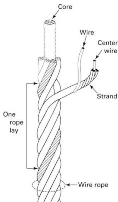
Figure 9-2.0-2 Wire Rope
