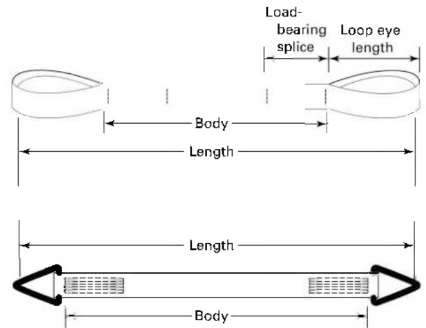
Figure 9-5.0-2 Synthetic Webbing Sling Nomenclature
