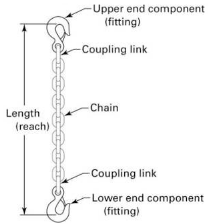
(b) Single-Leg Sling Components
