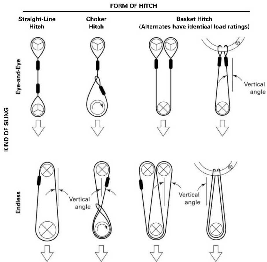
Figure 9-4.5-1 Hitch Types for Synthetic Rope Slings
