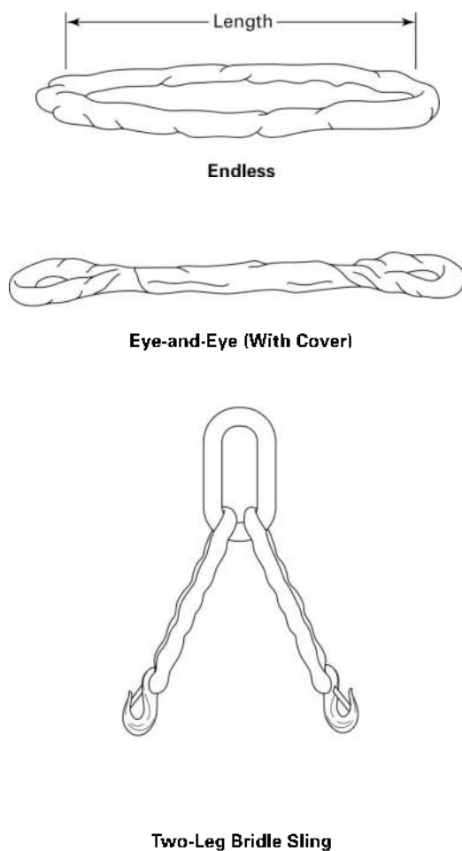
Figure 9-6.0-1 Polyester Roundsling Types
