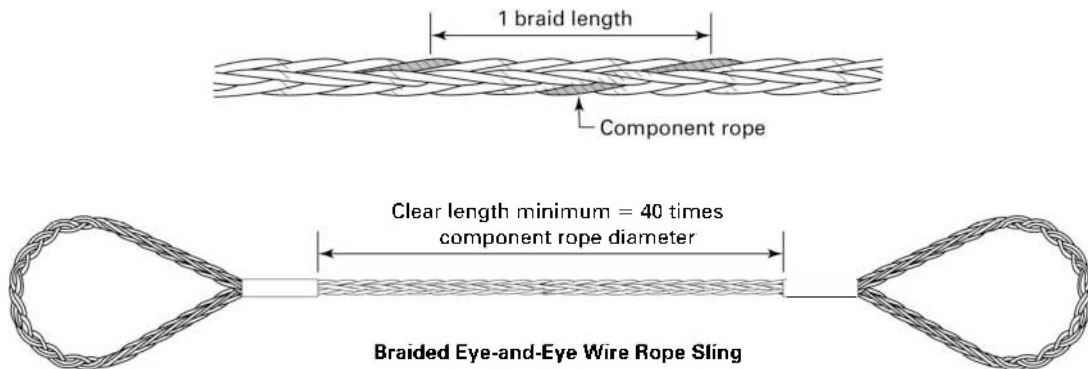
Figure 9-2.3.2-2 Minimum Braided Sling Length
