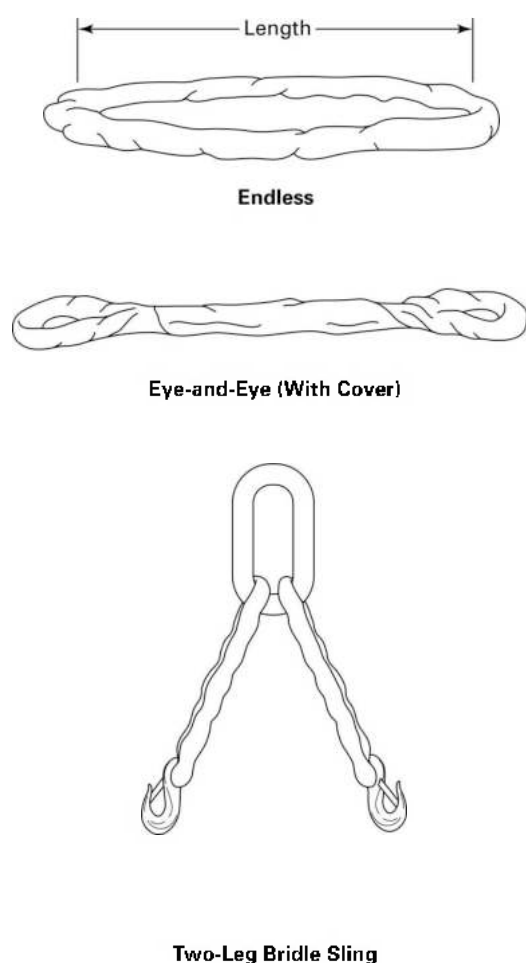
Figure 9-7.0-1 High Performance Roundsling Types
